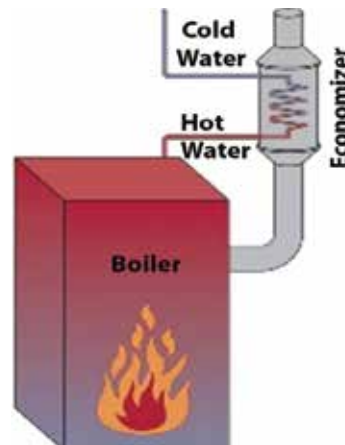
Economizer System
