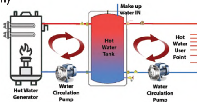
Hot Water Generation & Distribution
